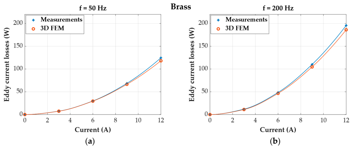
Figure 6. Measured and calculated eddy current losses in the brass clamping devices, where (a) at 50 Hz; (b) at 200 Hz.
