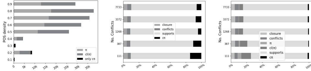
Figure 2: Proportion of assertions in each repair vs POS density [left]. Proportion of repair time for ABox u.5 , using Algorithm 4 [middle] and Algorithm 5 [right].
