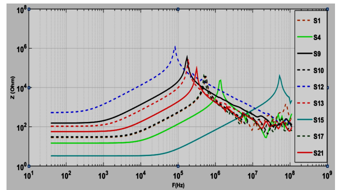
Figure 3. Frequency response of sensors made with wire diameter d = 0.1mm.
