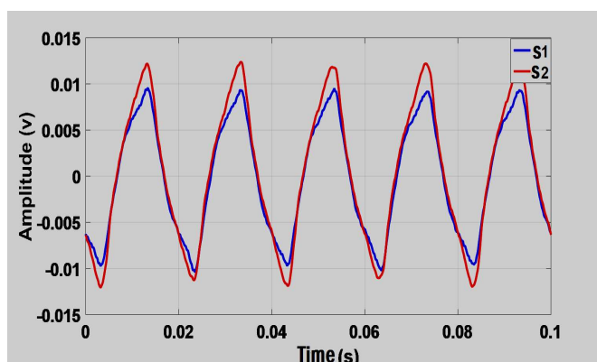
Figure 11. E.m.f induced in the sensors for a faulty machine.
