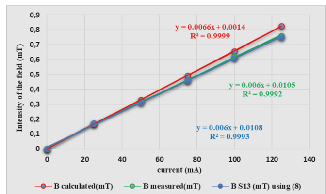
Figure 9. Linear intensity variation of the calculated magnetic field (B), measured by Tesla-meter and measured by S13 sensor.
