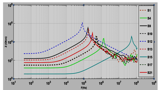
Figure 3. Frequency response of sensors made with wire diameter d = 0.1mm.
