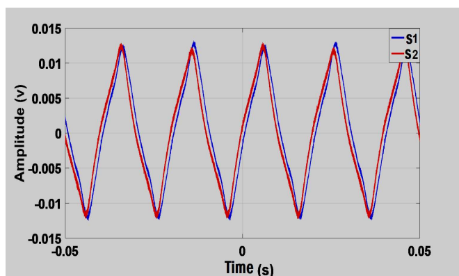
Figure 10. E.m.f induced in the sensors for a healthy machine.
