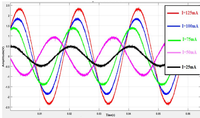
Figure 8. E.m.f induced for different values of the current in the magnetic field generator.
