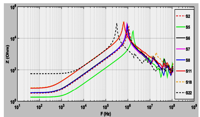
Figure 4. Frequency response of sensors made with wire diameter d = 0.3mm.
