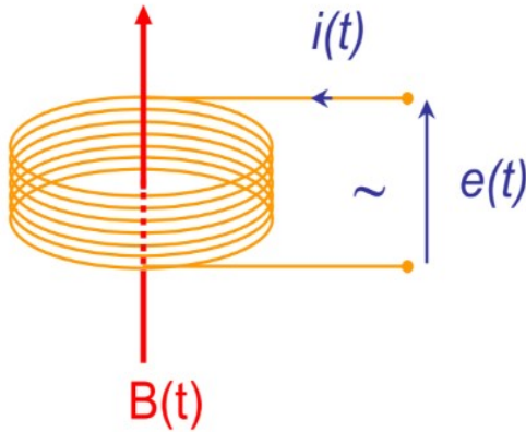
Figure 1. Schemes with ( e ) the voltage induced in a circuit which embraces the flux \phi ( t ) during the duration dt .
