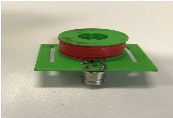
Figure 2. Coil sensor developed in the laboratory for the experimental investigations.
