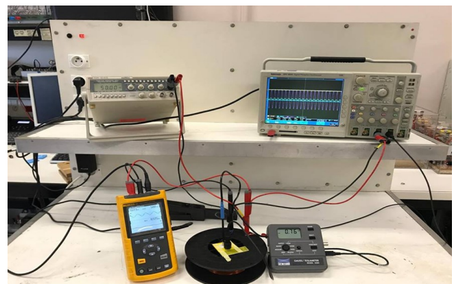
Figure 7. Field generator developed for testing the sensors.
