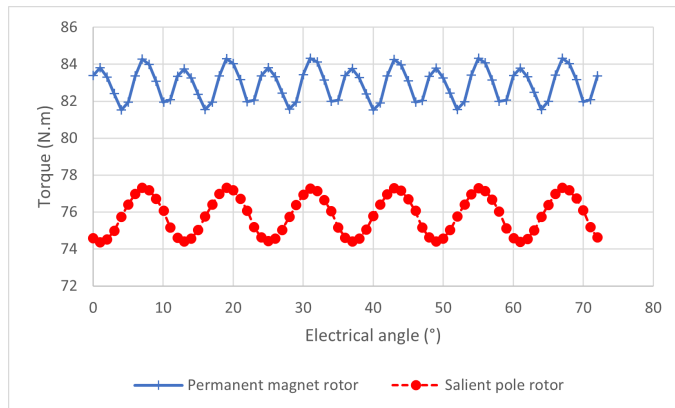
Fig. 6. Torque comparison at the rated operating conditions
