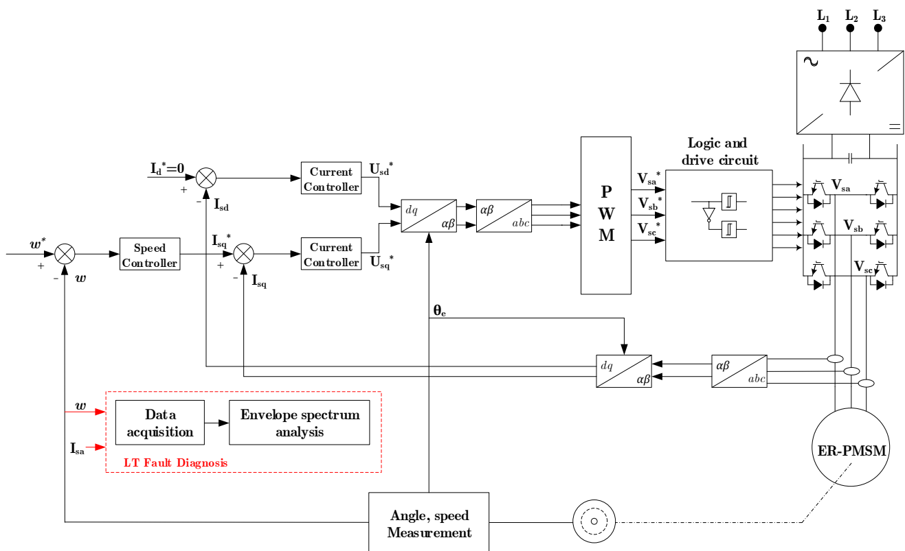
Figure 15. The flow chart of the proposed strategy.
