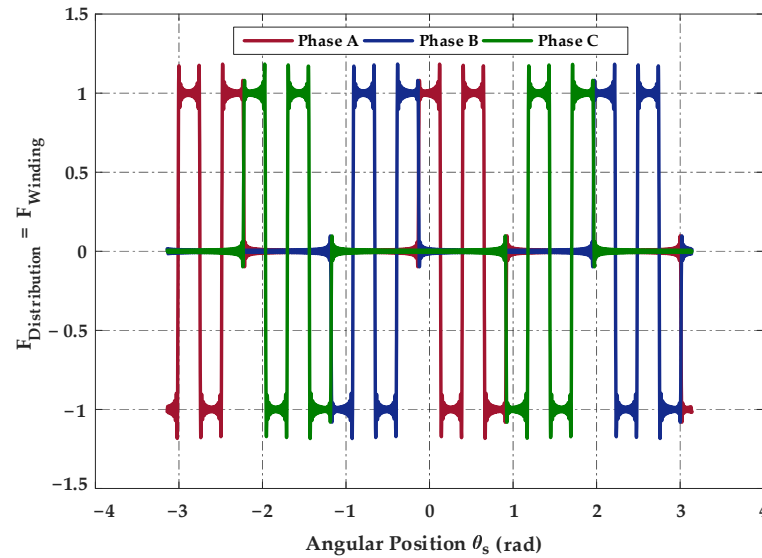
Figure 2. Distribution function of ER-PMSM.
