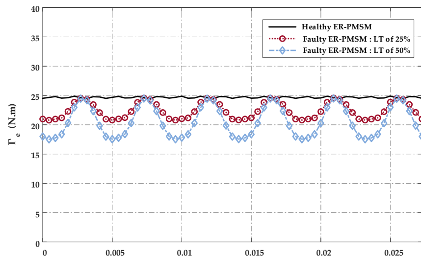
Figure 13. Electromagnetic torque comparison.
