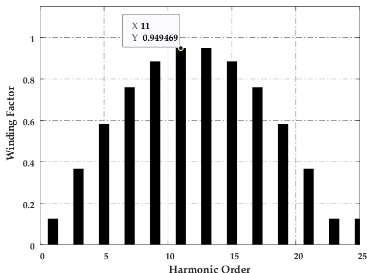
Figure 4. Harmonic spectrum of the winding factor.
