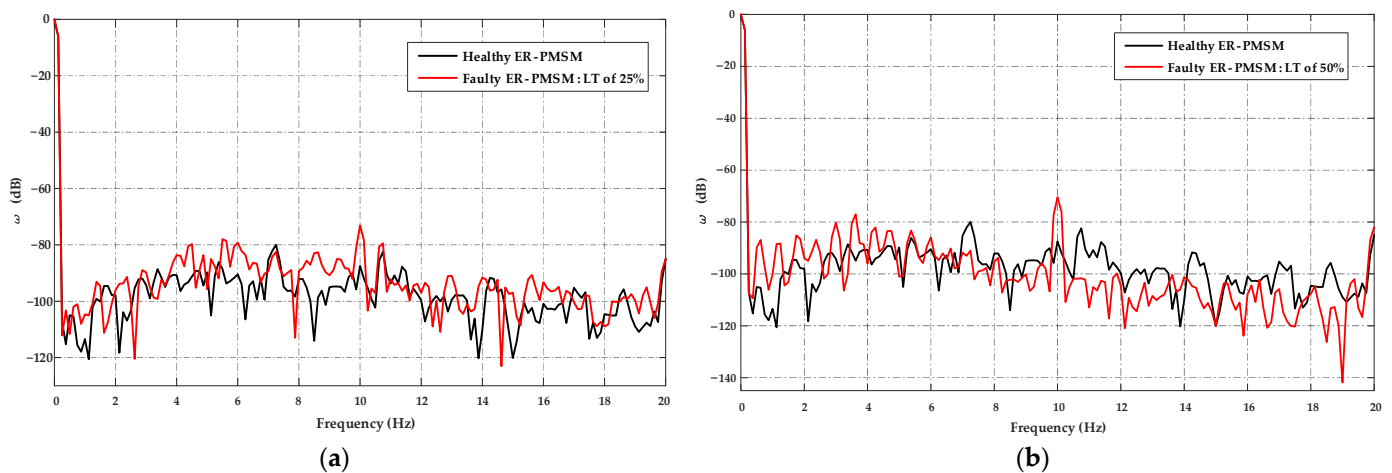
Figure 19. Experimental speed spectrum of the ER-PMSM at 8 Nm load and 600 rpm, in healthy and faulty conditions. (a) LTs fault of 25%; (b) LTs fault of 50%.
