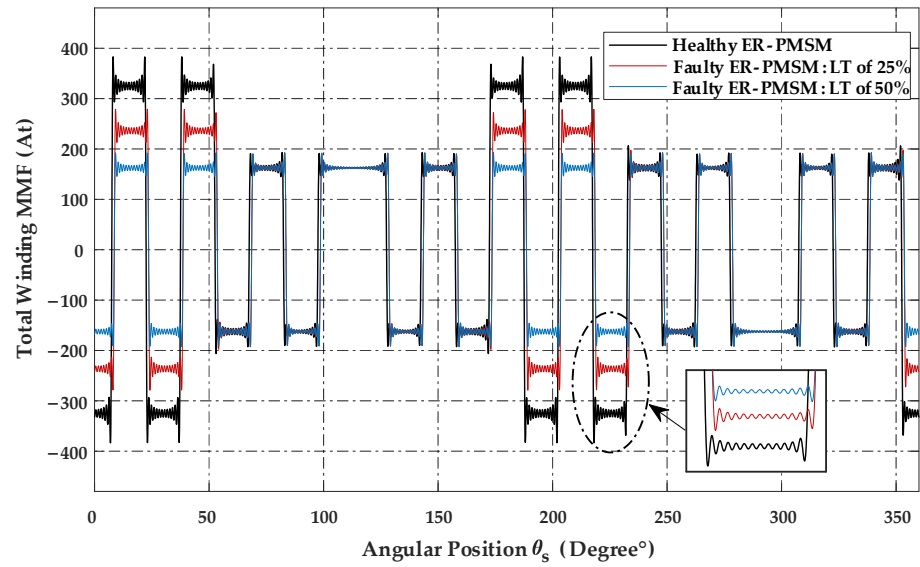
Figure 5. Healthy and faulty stator MMF distribution.
