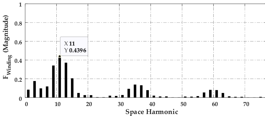
Figure 3. Harmonic spectrum of the winding function.
