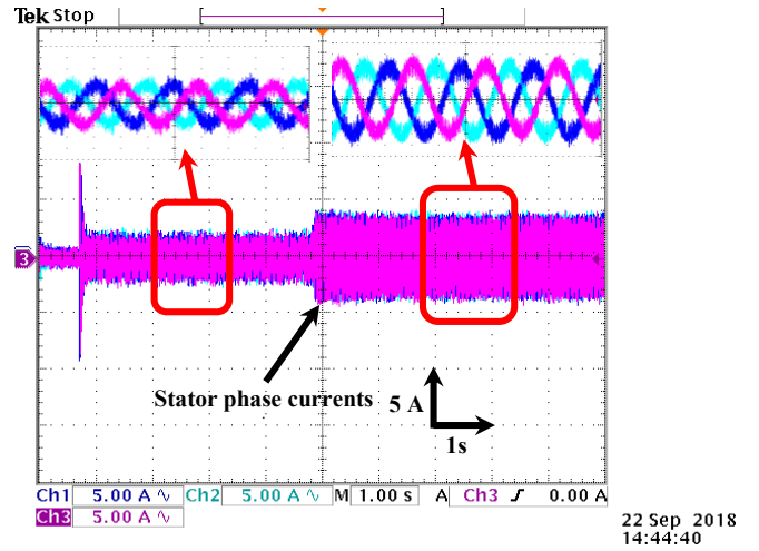
Fig. 6. Stator phase currents with rated load application
