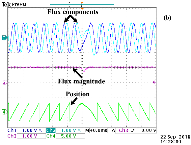
Fig. 4. Speed reversal tests, (a) speed and torque (b) flux components, flux magnitude and angel position.
