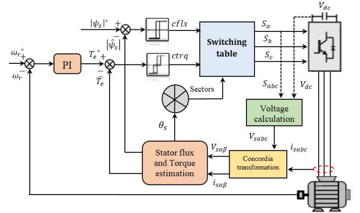
Fig.2 Global diagram of the switching table-based direct torque control.
