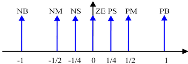
FIGURE 3 TS-FLC output membership functions [Color figure can be viewed at wileyonlinelibrary.com]
