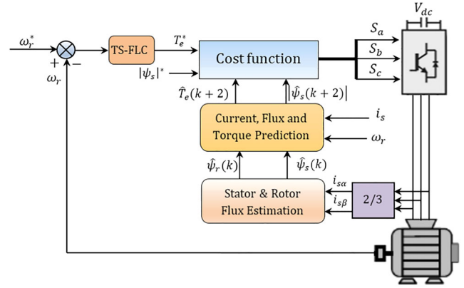
FIGURE 4 Block diagram of predictive torque control with T-S fuzzy logic speed controller for IM drive [Color figure can be viewed at wileyonlinelibrary.com]
