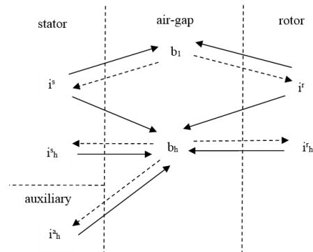
Fig. 5. Interactions between stator, rotor and auxiliary windings.
