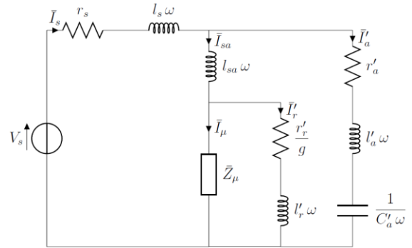
Fig. 4. Equivalent single-phase diagram.
