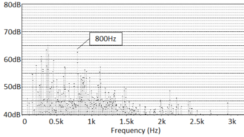
Fig. 11. Acoustic pressure level of the loaded machine at 1 meter, with three 107μF capacitors star connected.
