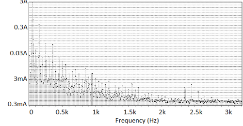
Fig. 12. Stator current spectrum without and with capacitors (scale in dB).
