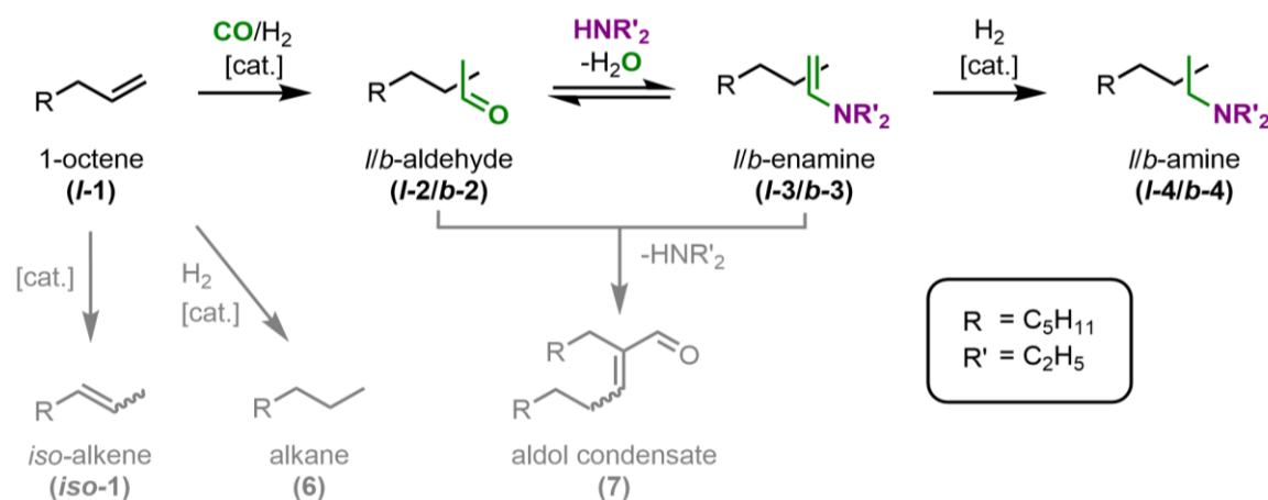
Figure 4: Reaction network for the hydroaminomethylation of 1-octene (I-1) with diethylamine (DEA) to the desired linear tertiary diethyl octylamine (I-4)
