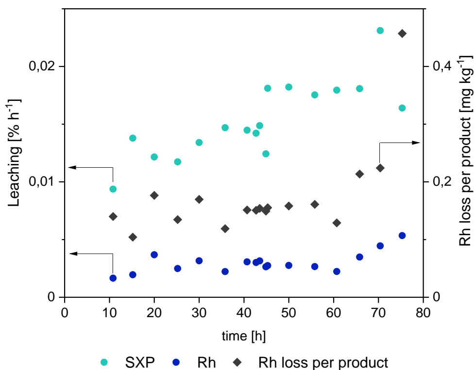
Figure 10: Leaching results of catalysts and ligand over reaction time. Leaching corresponds to % of the initial rhodium and sulfoXanphos mass.
