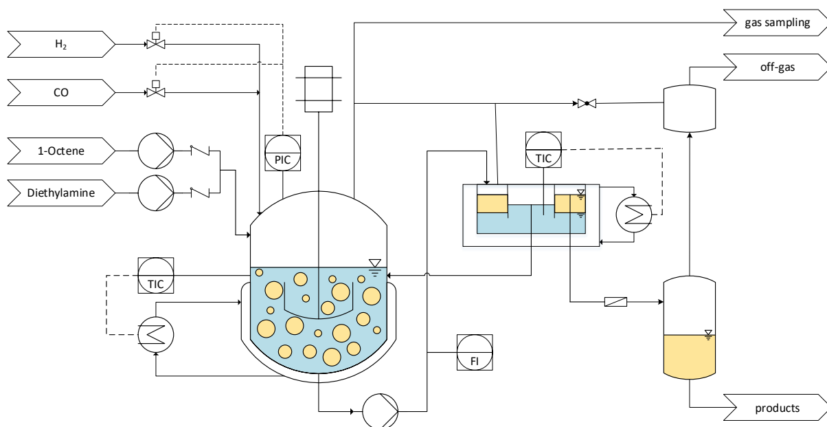
Figure 11: Flowchart of the commissioned and continuously operated miniplant.
