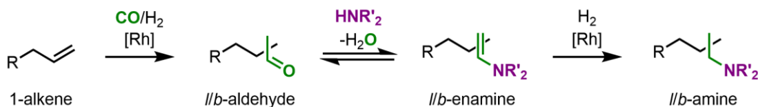
Figure 3: General scheme of the hydroaminomethylation based on a 1-alkene and a secondary amine.
