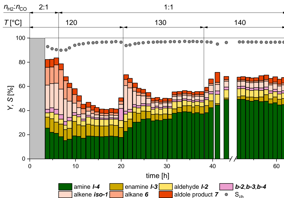
Figure 8: Reaction profiles for the continuous operated hydroaminomethylation of 1-octene with diethylamine at varying reaction temperature and gas ratio. Conversion equals sum of all yields. Yields are calculated based on GC- FID analysis of product stream with dibutylether as internal standard. Conditions: t = 2.2 h; p = 35 bar;
