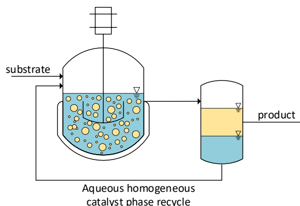
Figure 1: Basic process design for the recycling of homogeneous catalysts using aqueous biphasic reaction systems
