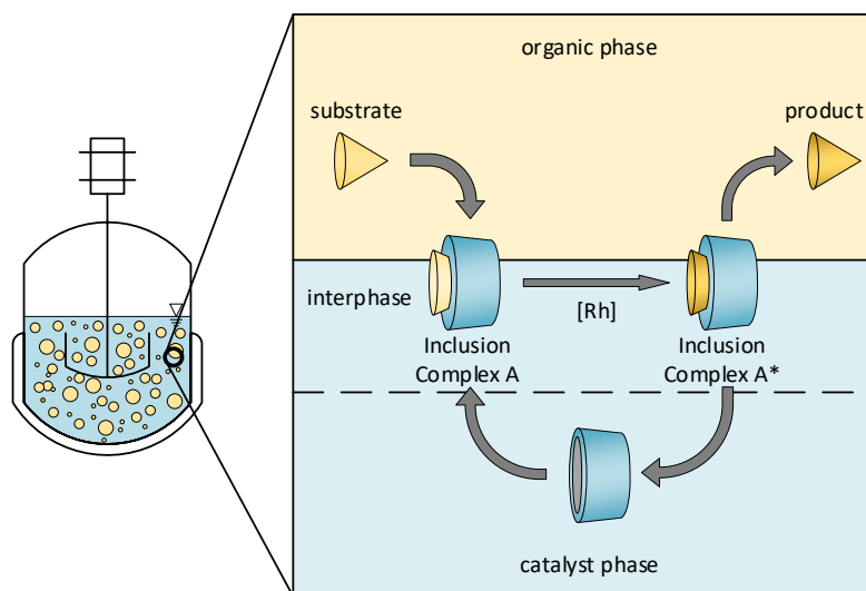
Figure 2: Proposed mechanism for cyclodextrin mediated reaction systems. [21]
