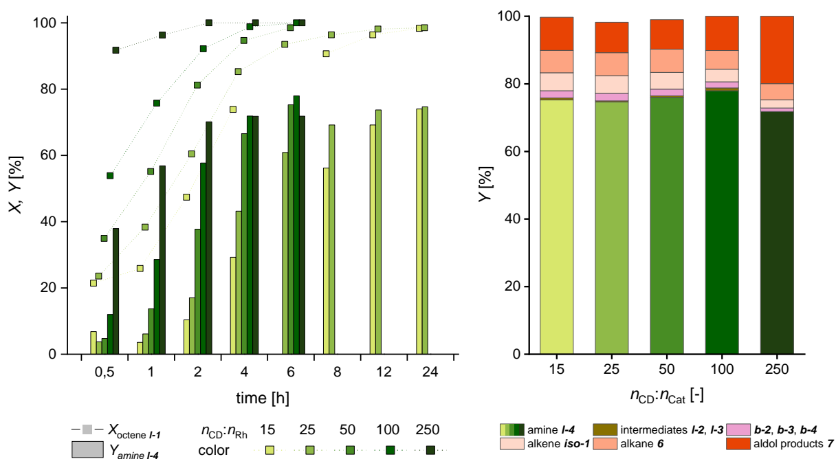
Figure 5: Conversion ( X ) and yield ( Y ) of I-1 over time (left) as well as product distribution (right) at full conversion of the HAM in dependency of the CD to catalyst ratio (Reaction time from left to right: 24 h, 12 h, 6 h, 6 h, 4 h).
