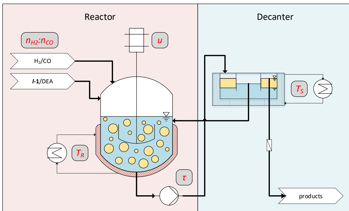
Figure 6: Conceptual flowsheet of the operated miniplant. Parameters which are varied in the continuous experiments are noted in gray boxes.
