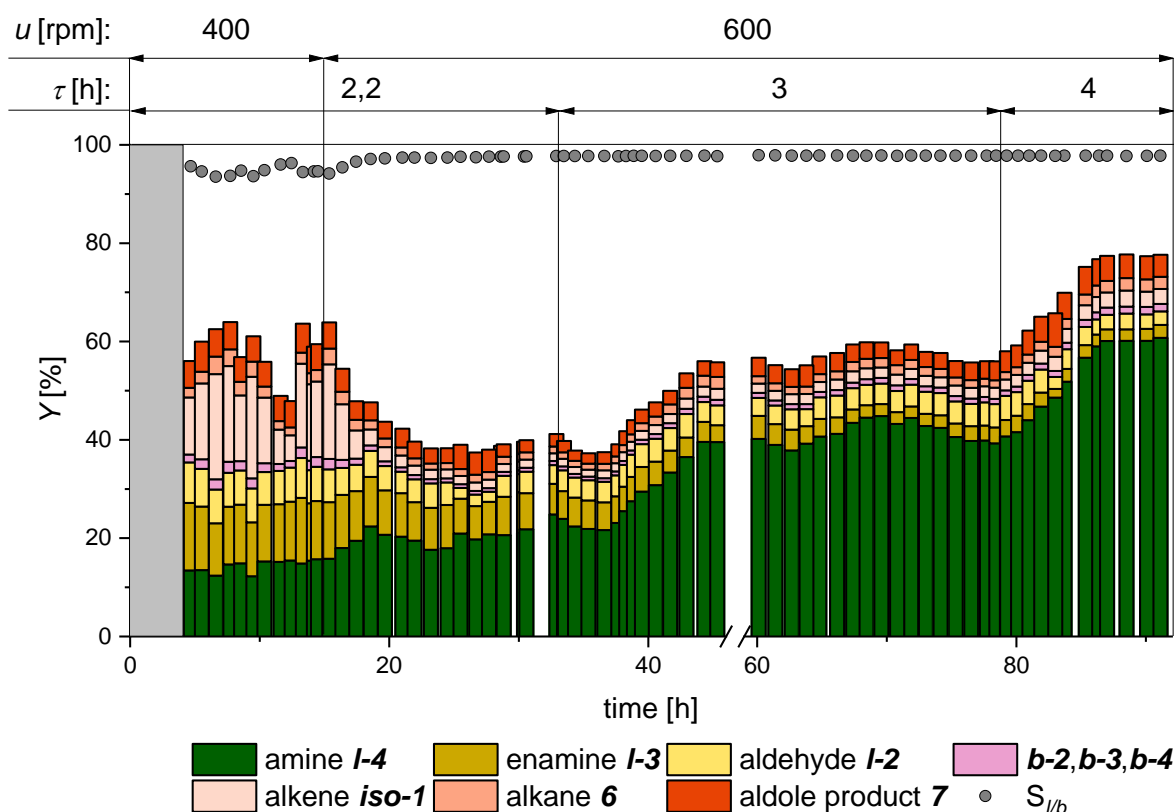
Figure 7: Reaction performance for the continuously operated hydroaminomethylation of 1-octene with diethylamine. Conversion equals sum of all yields. Yields are calculated based on GC-FID analysis of product stream with dibutylether as internal standard. Conditions: T = 120\text{ }^{\circ}\text{C} ; p = 30\text{ bar} ; u = 400\text{ to }600\text{ rpm} ; V_{\text{Reactor}} = 2100\text{ ml} , V_{\text{liq.}} = 770\text{ ml} ; n_{\text{H}_2}/n_{\text{CO}} = 1:1 ; c_{\text{Rh,aq,0}} = 3.2\text{ mmol L}^{-1} ; n_{1\text{-alkene}}:n_{\text{Rh}} = 500 ; n_{\text{CD}}/n_{\text{Cat.}} = 100 ; n_{\text{P}}/n_{\text{Rh}} = 7 ; n_{\text{DEA}}/n_{1\text{-Alkene}} = 1.5 ; \varphi = 0.2 ; \tau = 2.2\text{ h to }4\text{ h} ; preforming: T = 120\text{ }^{\circ}\text{C} ; p = 35\text{ bar} ; n_{\text{H}_2}/n_{\text{CO}} = 1:1 ; u = 800\text{ rpm} ; t > 12\text{ h} .
