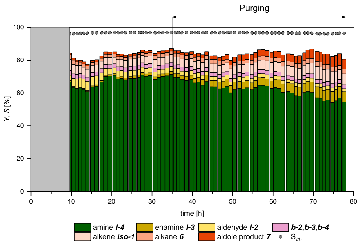
Figure 9: Yields over time for the continuously operated hydroaminomethylation of 1-octene with diethylamine. Conversion equals sum of all yields. Yields are calculated based on GC-FID analysis of product stream with dibutylether as internal standard. Conditions: t = 4 h; T = 140 °C, p = 35 bar; n_{H_2}/n_{CO} = 1:1 ; u = 600 rpm; c_{Rh,aq,0} = 3.2 mmol L -1 ; n_{1-alkene}:n_{Rh} = 500 ; n_{CD}:n_{Rh} = 100 ; n_P:n_{Rh} = 7 ; n_{DEA}:n_{1-alkene} = 1.5 ; \varphi = 0.2 ; preforming: T = 120 °C; p = 35 bar; n_{H_2}/n_{CO} = 1:1 ; u = 800 rpm; t > 12 h.
