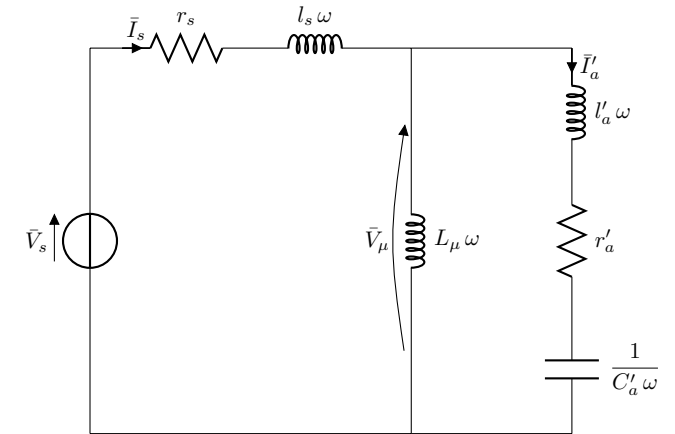
Fig. 4. Single-phase two-winding equivalent circuit
