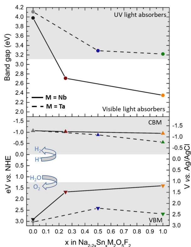
Figure 6: Evolution of band gap (top panel) and band edge position (bottom panel) as a function of x in \text{Na}_{2-2x}\text{Sn}_x\text{M}_2\text{O}_5\text{F}_2 series obtained from UV-vis diffuse reflectance spectra and Mott-Schottky measurements.
