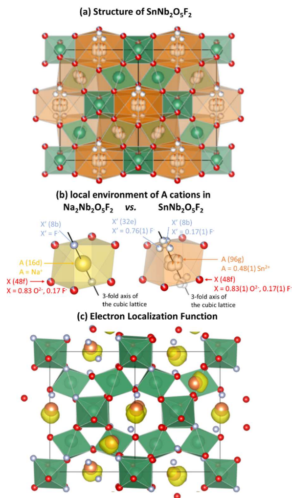
Figure 3: Structure of \text{SnNb}_2\text{O}_5\text{F}_2 (a) and comparison of its local A site environment with the one observed in \text{Na}_2\text{Nb}_2\text{O}_5\text{F}_2 (b). Relaxed Structure obtained from DFT calculation and localization of the \text{Sn}^{2+} lone pair obtained with ELF (c).
