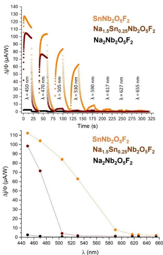
Figure 7: Photocurrent density as a function of wavelength in \text{Na}_{2-2x}\text{Sn}_x\text{Nb}_2\text{O}_5\text{F}_2 ( \Phi = 20 \text{ mW}/\text{cm}^2 , V_{\text{bias}} = 0.8 V vs. Ag/AgCl in a 0.1 M aqueous solution of \text{Na}_2\text{SO}_4 as electrolyte).
