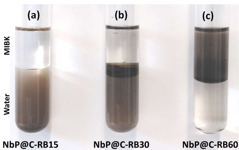
Figure 9. Photographs displaying the distribution of the NbPC@RB x samples [ x = 15 (a), 30 (b) and 60 (c)] in a mixture of water-MIBK. Experimental conditions: 10 mg of catalyst; 3 mL of MIBK; 3 mL of water. The mixture was treated under ultrasound for 5 minutes at room temperature and left to stand under static conditions until complete decantation.
