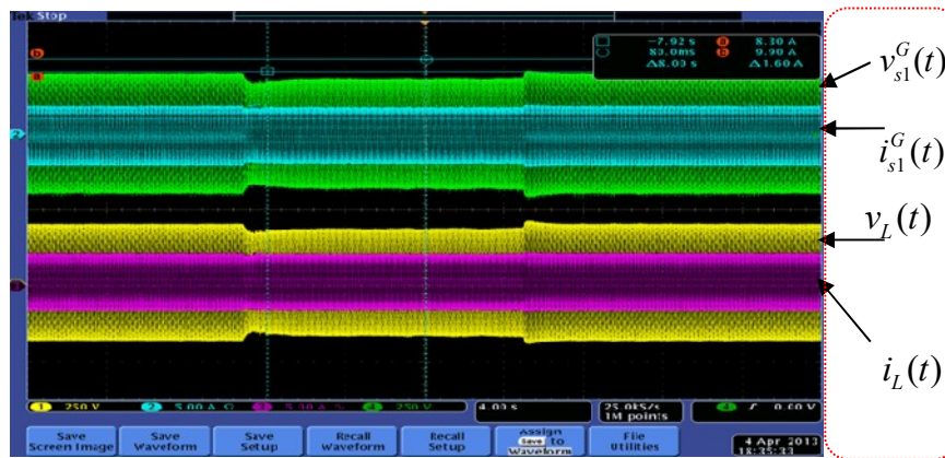
435 Fig. 26. Wave forms of recording signals : top lines show voltage and current lines measured at the 436 SEIG output, bottom lines show voltage and current lines of TCR system for wind speed switching 437 from V_w = 13\text{m/s} to V_w = 12\text{ m/s} and return to 13\text{ m/s} .
