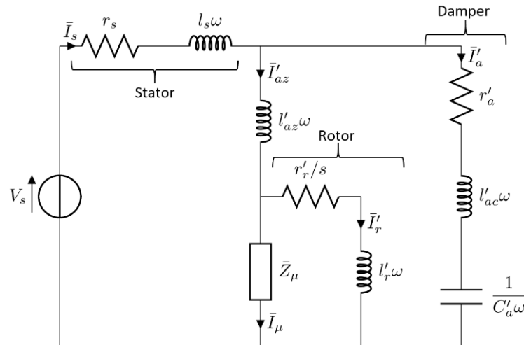
Fig.2. Single-phase equivalent diagram of the machine with damper windings.
