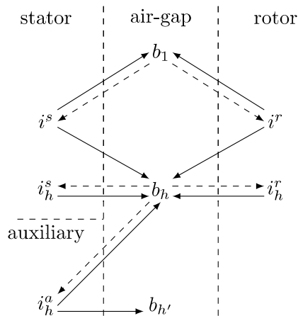
Fig. 5. Interactions between stator, rotor and auxiliary windings.
