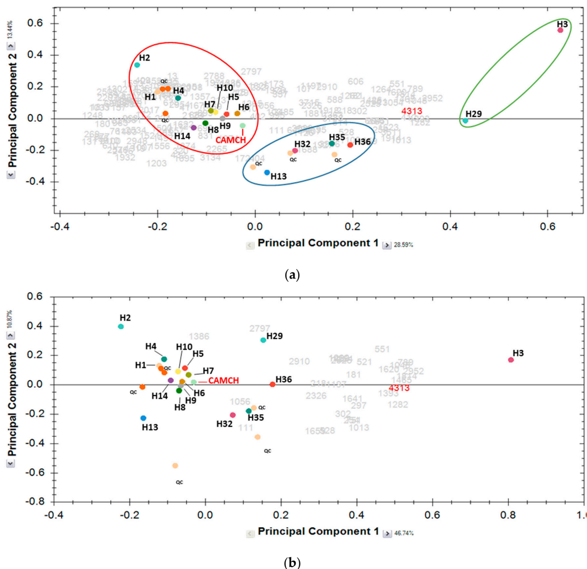
Figure 3. Principal component analysis of the most abundant identified peptides corresponding to the commercially available, unknown milk casein hydrolysate (CAMCH) and the 16 hydrolysates of (a) milk protein liquid fraction enriched in micellar caseins (ratio micellar caseins/whey proteins (92:8)) and (b) the 32 peptides (depicted in grey numbers) most abundant in H3 than in other hydrolysates (H13, H2, H14, H5, H1, H32, H4, H29, H36, and CAMCH). Principal components #1 and #2 of A explain 28.92% and 13.56% of variance, while principal components #1 and #2 of B explain 47.12% and 10.98% of variance, respectively. Grey numbers correspond to identified peptides displaying a mass signal intensity > 10^4 , while red number corresponds to one peptide of the H3 hydrolysate displaying the greatest fold change (infinity). Color circles are hand-marked to facilitate understanding and have no statistical significance.
