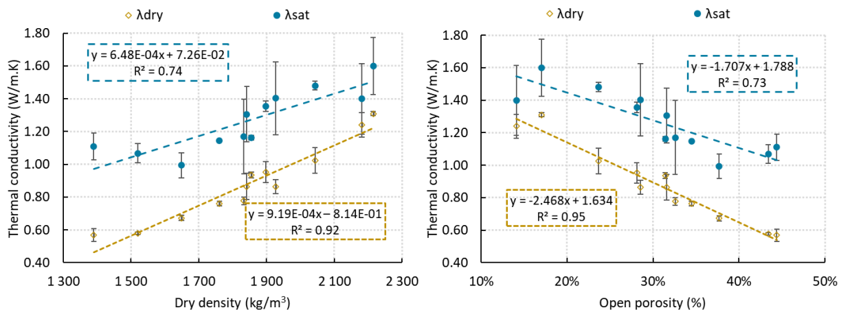
Fig. 10 Thermal conductivity as a function of density and porosity
