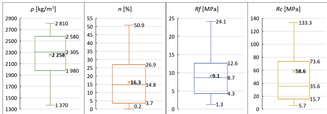
Fig. 1 The extent of mechanical properties of limestone
