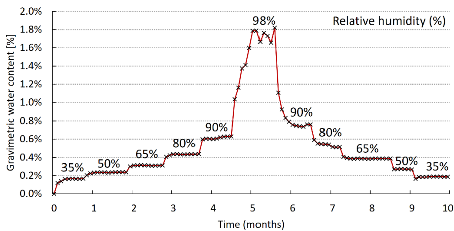
Fig. 5 Example of experimental stages (NOY stone)
