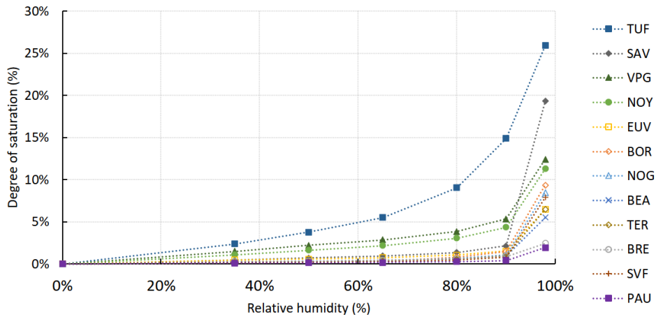
Fig. 6 Sorption isotherms of the twelve samples
