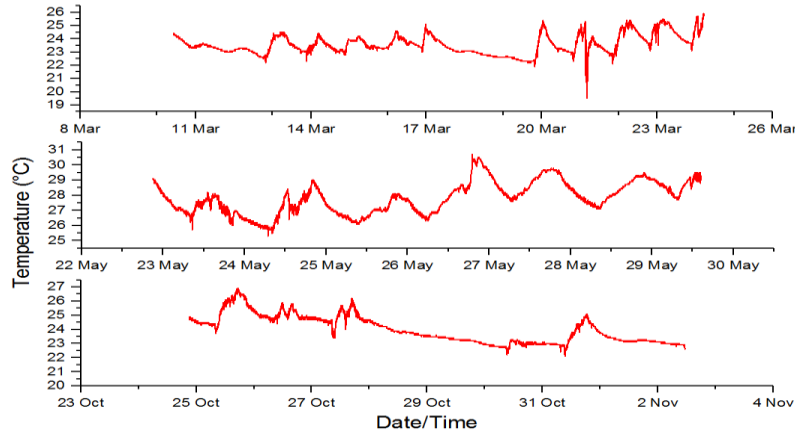
Fig. 9. Indoor temperatures during measurement campaigns.
