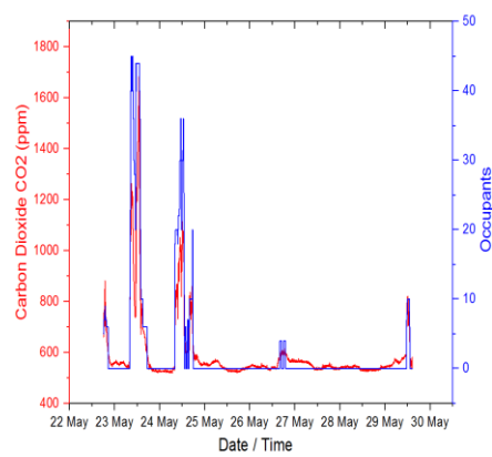
Fig. 5. CO 2 -concentrations and occupancy rate during the second period of IAQ measurement.
