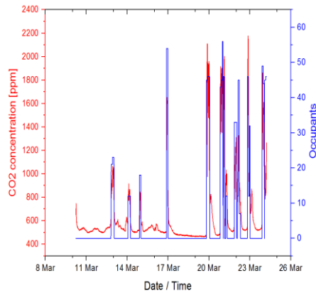
Fig. 4. CO 2 -concentrations and occupancy rate during the first period of IAQ measurement.
