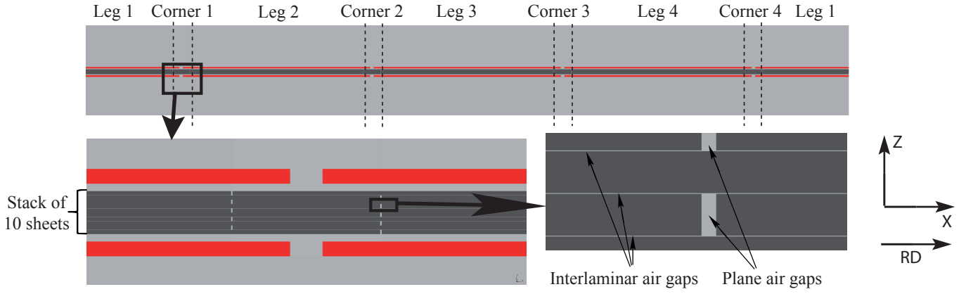
Fig. 5. Model for performing the Finite Element simulation of schematic outline transformer
