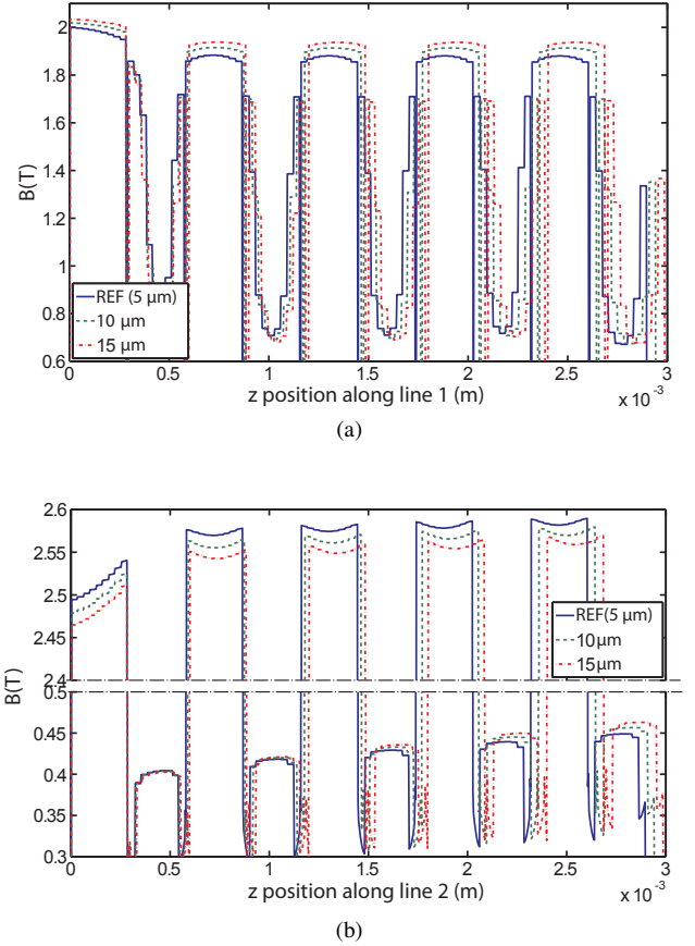
Fig. 7. Simulation results with homogeneous interlaminar air gaps along the line 1 (a) and the line 2 (b)
