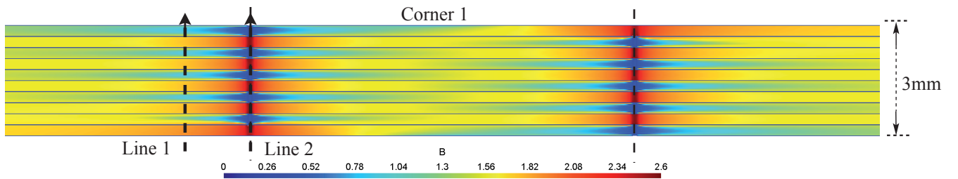
Fig. 6. Magnetic flux density distribution when all the interlaminar air gaps have the same thickness ( 5 \mu\text{m} )
