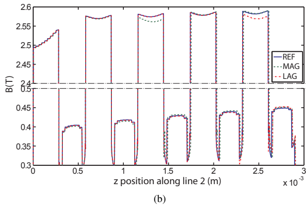
Fig. 8. Simulation results with one air gap thickness different from the others along the line 1 (a) and the line 2 (b)
