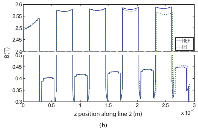
Fig. 9. Simulation results with non-homogeneous interlaminar air gaps along the line 1 (a) and the line 2 (b)
