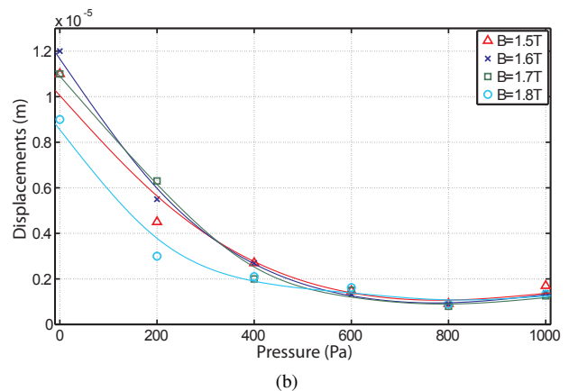
Fig. 4. Displacements with the pressure and the flux density in the middle (a) and the interior (b) of the corner (measurements and trend curves)
