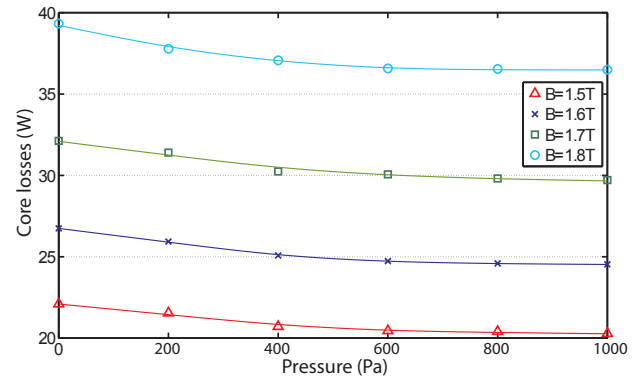
Fig. 3. Core losses variations with respect to the applied pressure and the flux density (measurements and trend curves)
