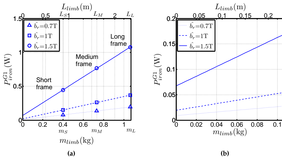
Figure 4. (a) Variations of P_{iron} with m_{limb} for \hat{b} = 0.7\text{T} , \hat{b} = 1\text{T} and \hat{b} = 1.5\text{T} for G1 steel (b) Zoom near the abscissa 0.
