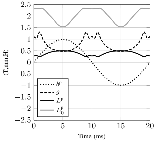
Fig. 7. Variations with time of b^P , g , L^P , L_0^P for V^P = 240 V and i^A = 20 A
