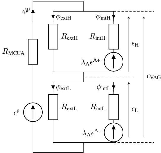
Fig. 4. Reluctance network
