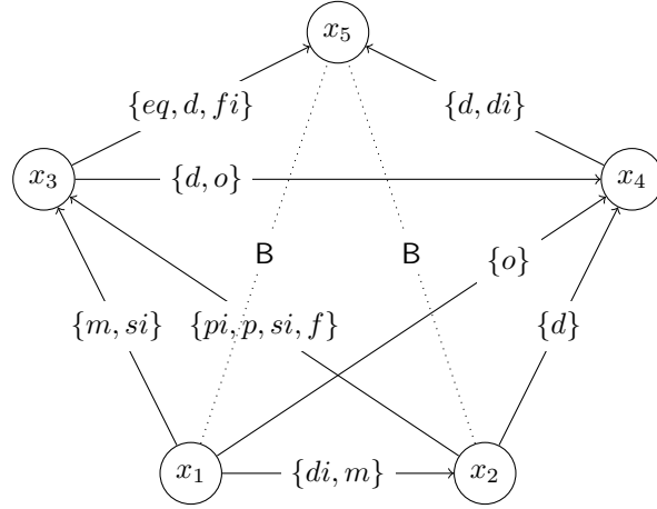
Figure 4: Given the QCN \mathcal{N} = (V, C) above and the graph G that results by removing the edge \{x_1, x_5\} from the complete graph on V , we have that \mathcal{N} is neighbourhood \overset{\circ}{G} -consistent (and neighbourhood \overset{\circ}{G} -consistent), but not \overset{\circ}{G} -consistent (or \overset{\circ}{G} -consistent)
