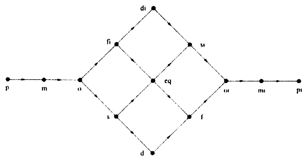
Figure 3: The interval lattice (\mathcal{B}_{int}, \leq) .
