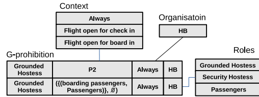
Figure 11: G-prohibition relation
