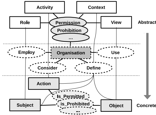
Figure 1: OrBAC model
