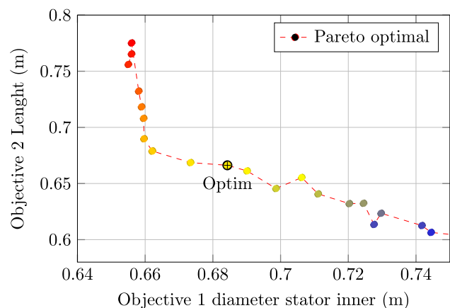
Figure 8: Pareto curve for two objectives about a design motor with iron cobalt electrical sheet steel.
