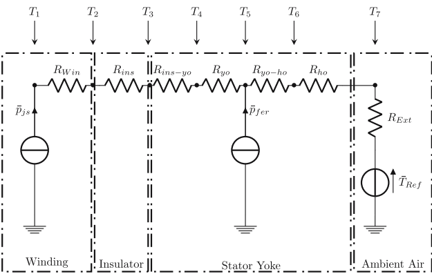
Figure 4: Simplified thermal circuit model.
