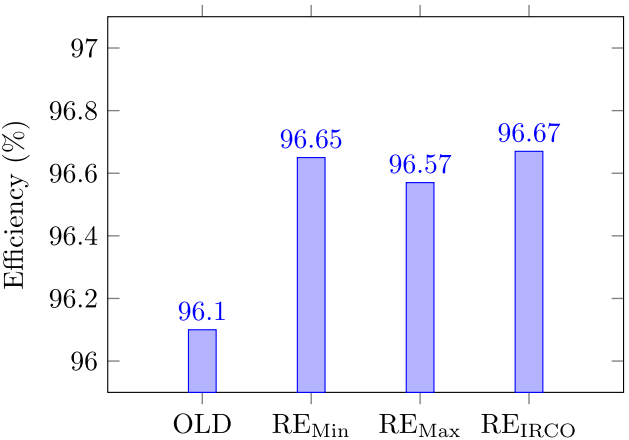
Figure 6: Efficiency of each configuration.
