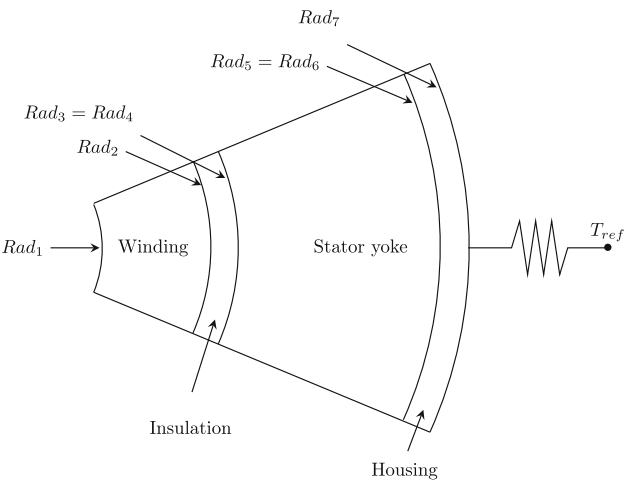
Figure 5: Simplified stator for the thermal model.
