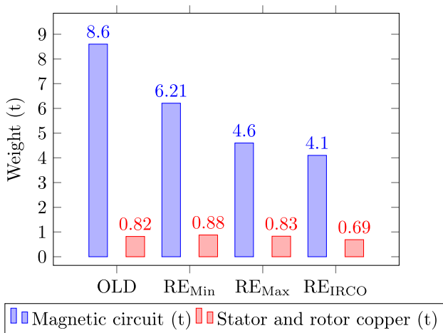
Figure 7: Weight of magnetic circuit and copper of each configuration.
