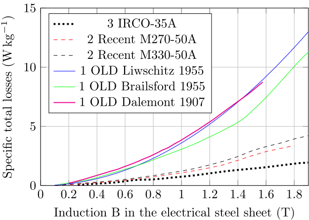
Figure 3: Electrical steel sheets quality comparison of specific total losses.
