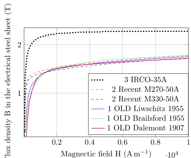
Figure 2: Electrical steel sheets quality comparison of B–H curves.
