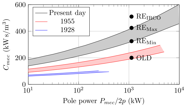
Figure 1: Evolution of machine sizing constant C_{mec} based on empirical knowledge and a traditional know-how, for pole pairs two to six.
