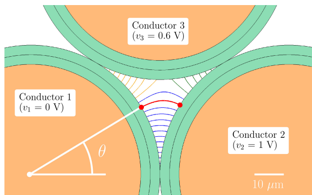
FIGURE 2. Calculated field lines in an air gap between three wires (wire radius is 40 \mu\text{m} , insulation thickness is 7 \mu\text{m} ), with a potential of 0.6 \text{ V} imposed on conductor 3. The field line and corresponding angle \theta where PDs are predicted to occur are highlighted. The voltage drop is calculated between the two red dots on the insulation surface.
