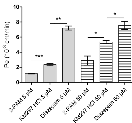
Figure 7. Endothelial permeability coefficient (Pe) of 2-PAM, KM297 HCl, and diazepam measured in the human in vitro BBB model at 5 and 50 \mu M. Values are presented as mean \pm SEM, n = 3 –12. Comparisons were performed using Mann–Whitney test between KM297 HCl and 2-PAM or diazepam. * p < 0.05 , ** p < 0.01 , *** p \leq 0.001 .
