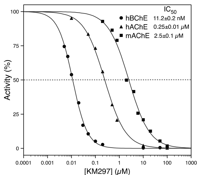
Figure 5. In vitro \text{IC}_{50} determination of KM297 HCl for hAChE, mAChE, and hBChE.
