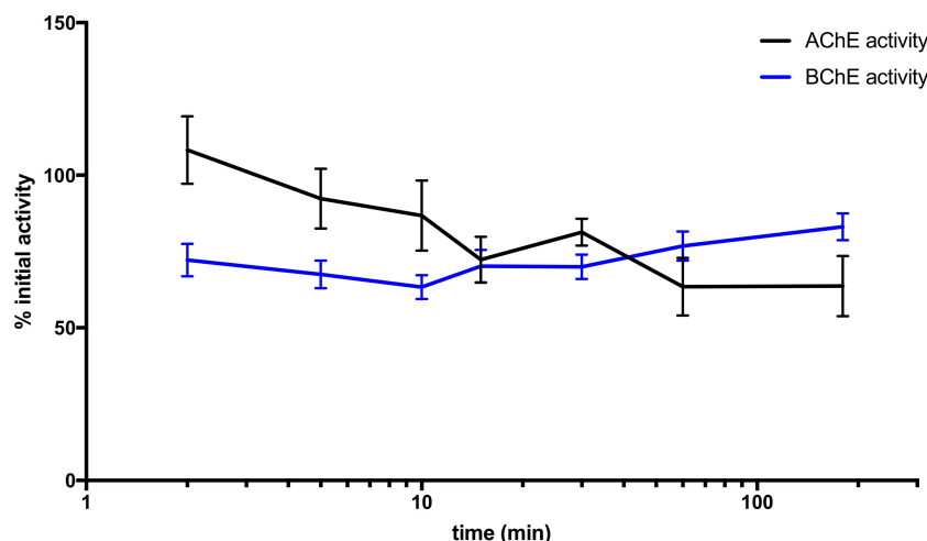
Figure 4. Mice blood AChE and BChE activity follow-up after an i.p. administration of 100 \mu\text{mol/kg} KM297 HCl ( n = 8\text{--}10 ). Blood samples were drawn at various time points (0, 2, 5, 10, 15, 30, 60, and 180 min) after treatment, and AChE and BChE activity levels were measured. Values are presented as percentages of corresponding initial activity and points are means \pm SEM.
