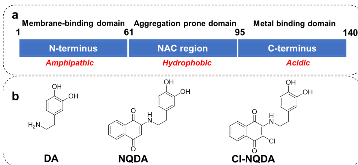
Figure 1. (a) Schematic structure of \alpha -Syn. (b) Chemical structures of DA, NQDA and Cl-NQDA.
