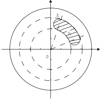
Figure 1: Round dyadic set \hat{S}_l
